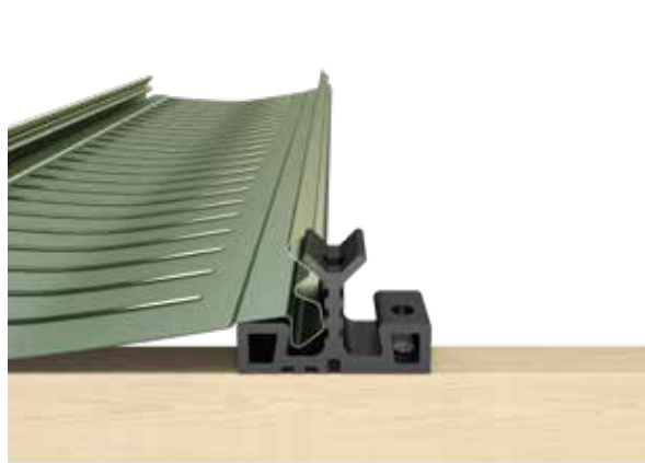
2 _ Incastro prima lastra / Push down first sheet
